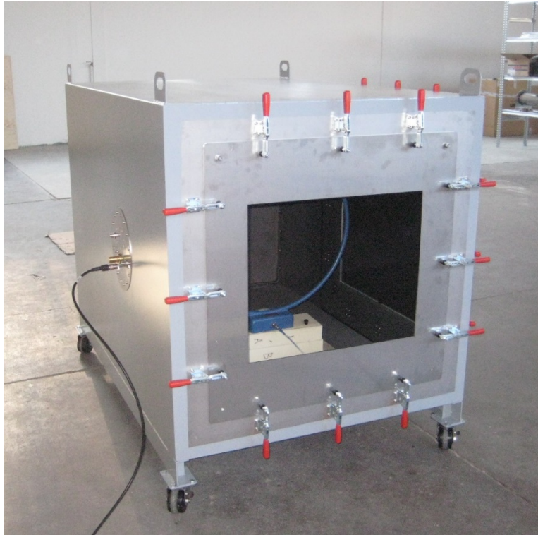
Test box L1xH1xW1,5m lined with flat anechoic absorbers
