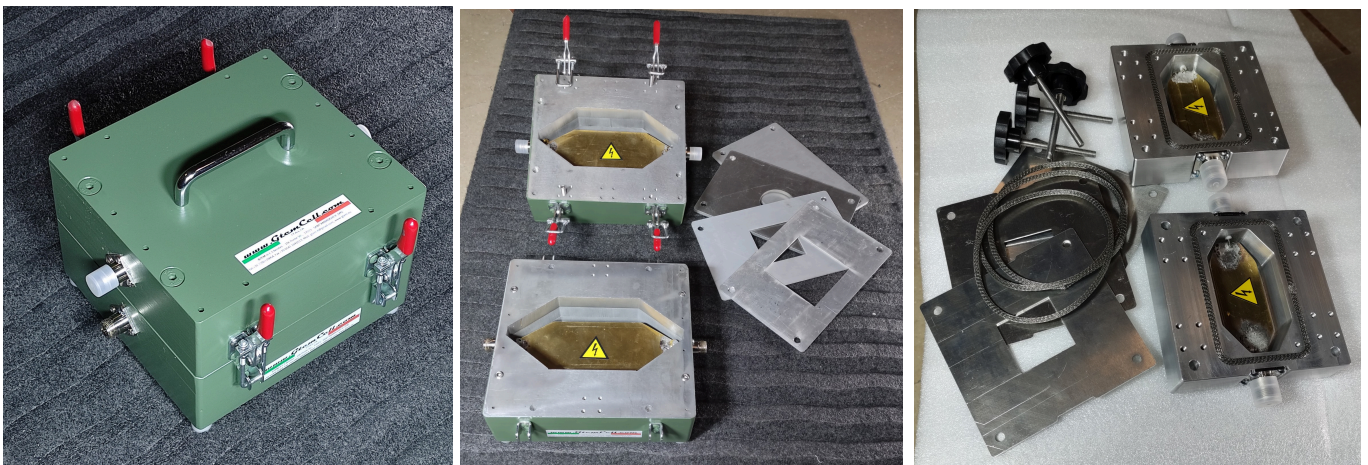
. D-TEM3000 and the half valves of the D-TEM6000 and D-TEM3000 open.
